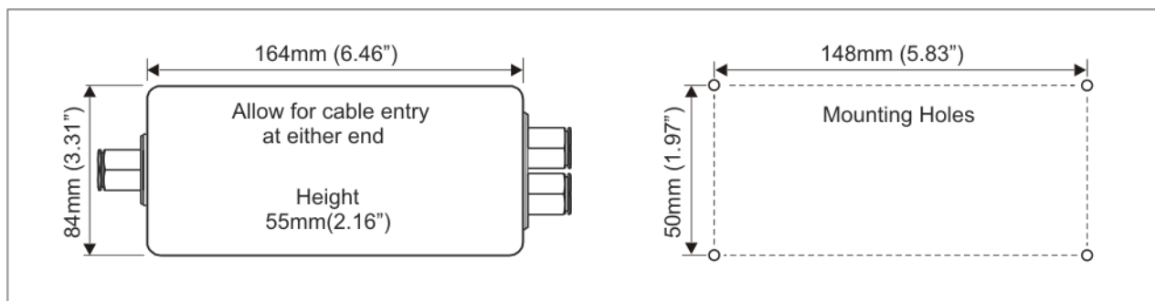
Figure 2.1 Dimensions
